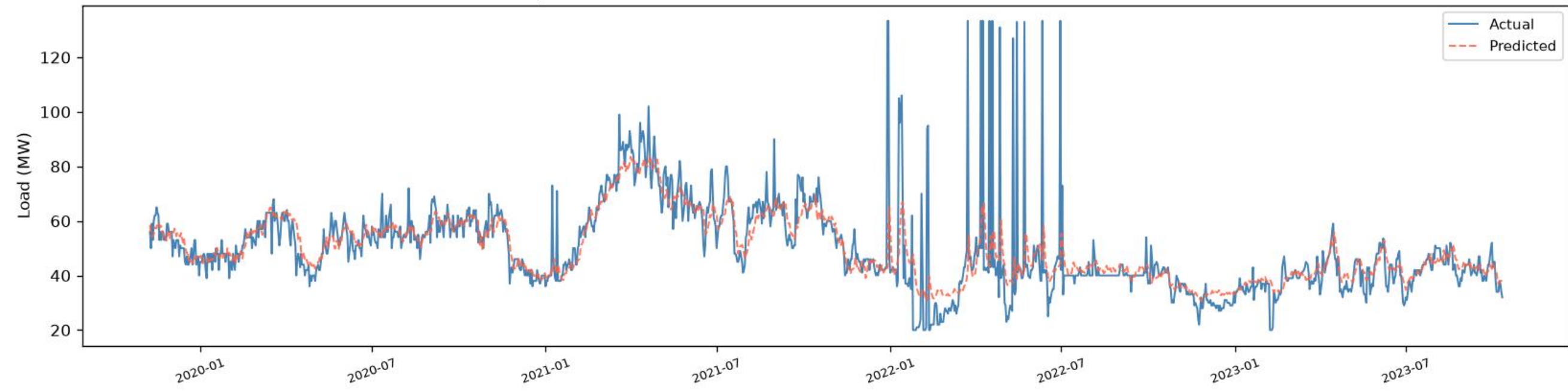
Ullon | BiLSTM - TRAIN (fit block) ( R^2=0.5624 , RMSE=10.76, MAE=5.14, n=1385)
