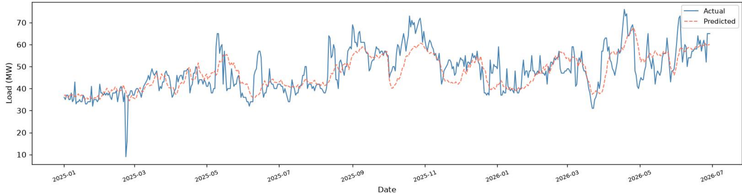
Ullon | CNN+BiGRU+BiLSTM - TEST ( \geq 2025 ), one-day-ahead ( R^2=0.5267 , RMSE=6.69 , MAE=4.95 , n=536 )
