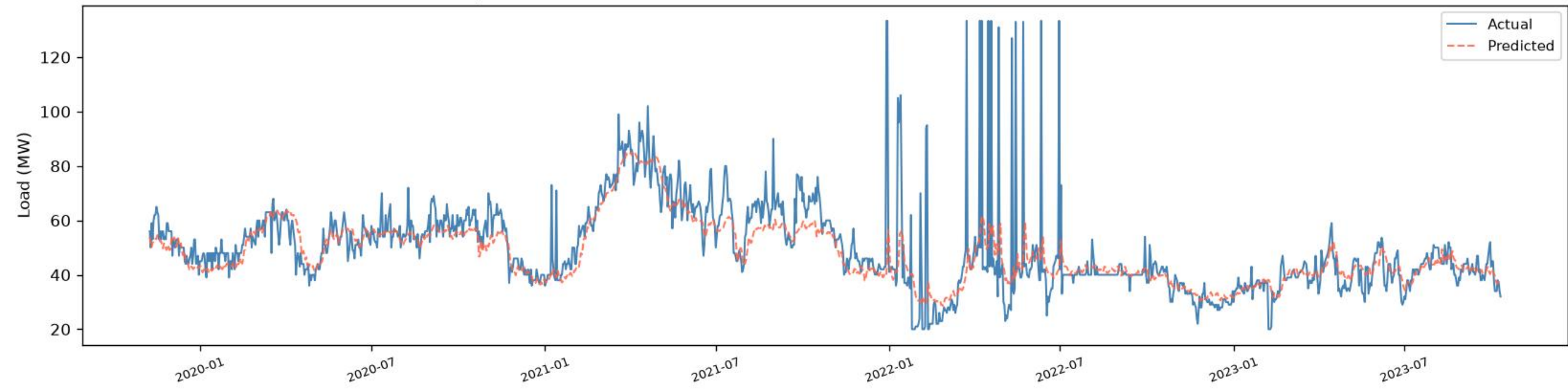
Ullon | CNN+BiGRU+BiLSTM - TRAIN (fit block) (R2=0.5361, RMSE=11.07, MAE=5.58, n=1385)
