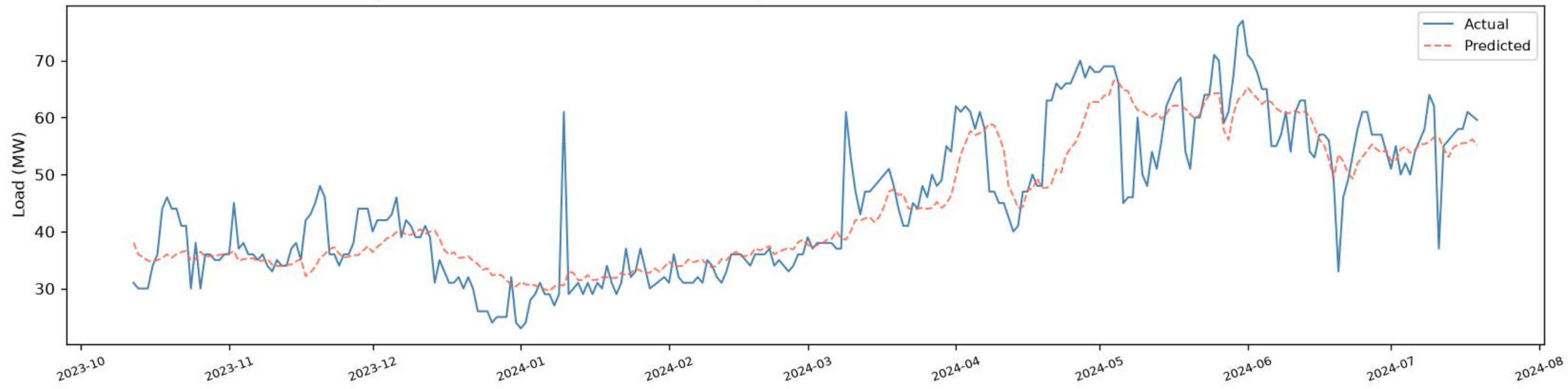
Ullon | CNN+BiGRU+BiLSTM - VALIDATION (chronological, before test) ( R^2=0.7600 , RMSE=6.35 , MAE=4.52 , n=272 )
