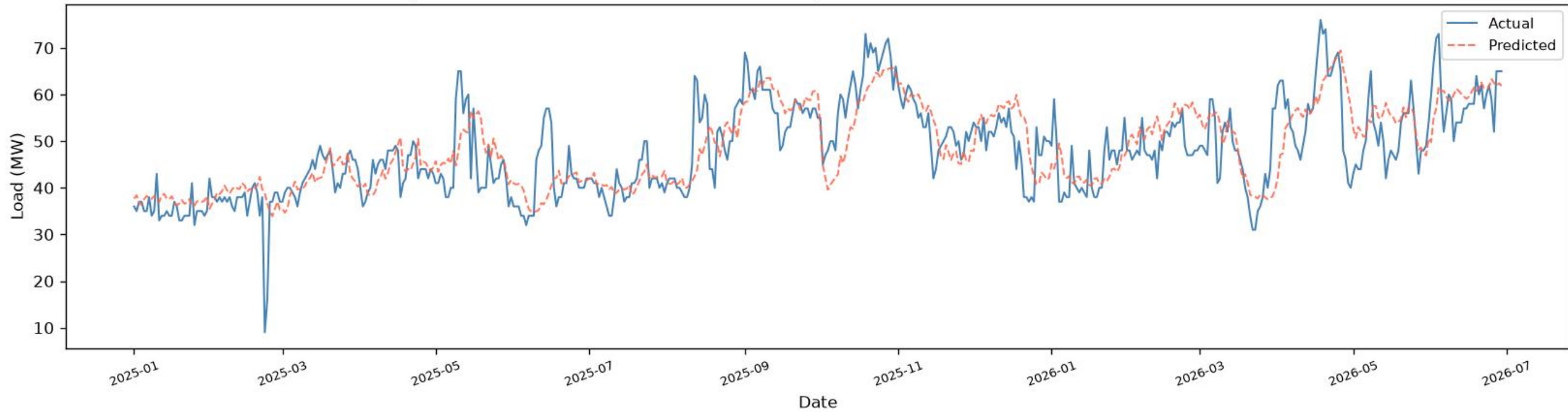
Ullon | CNN+BiLSTM+BiGRU - TEST ( \geq 2025 ), one-day-ahead ( R^2=0.5603 , RMSE=6.45 , MAE=4.76 , n=536 )
