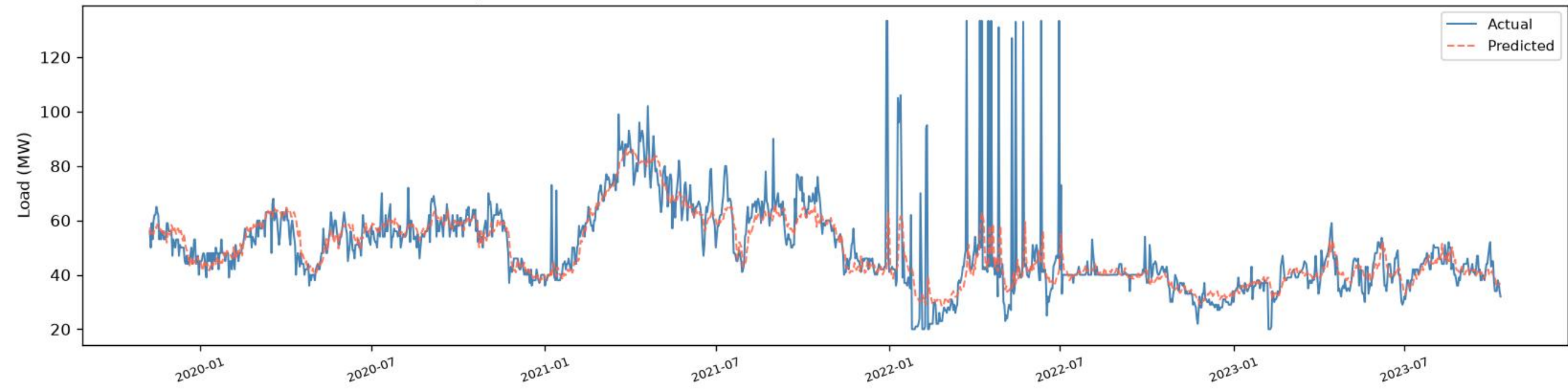
Ullon | CNN+BiLSTM+BiGRU - TRAIN (fit block) (R2=0.5576, RMSE=10.81, MAE=5.08, n=1385)
