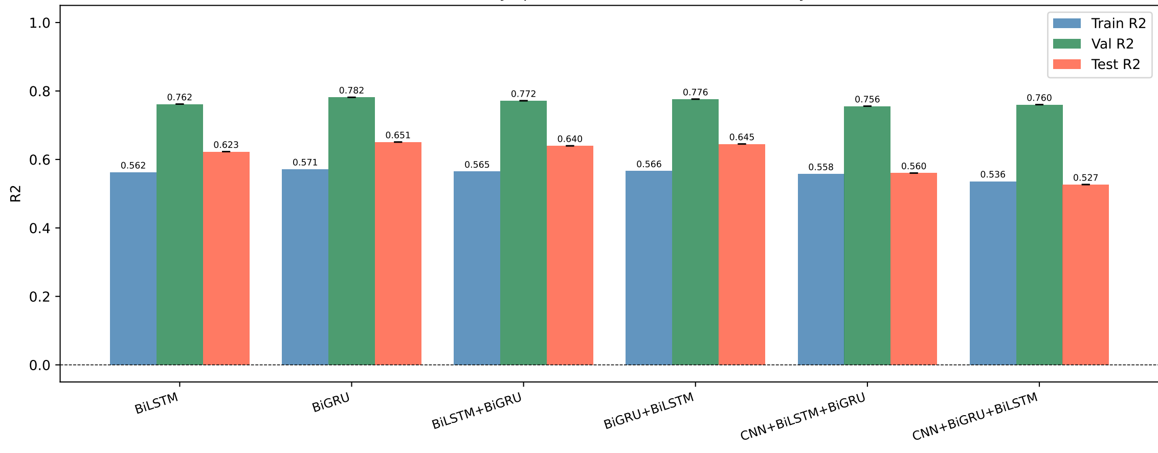
Ullon - R2 by split (model selection uses VAL only)
