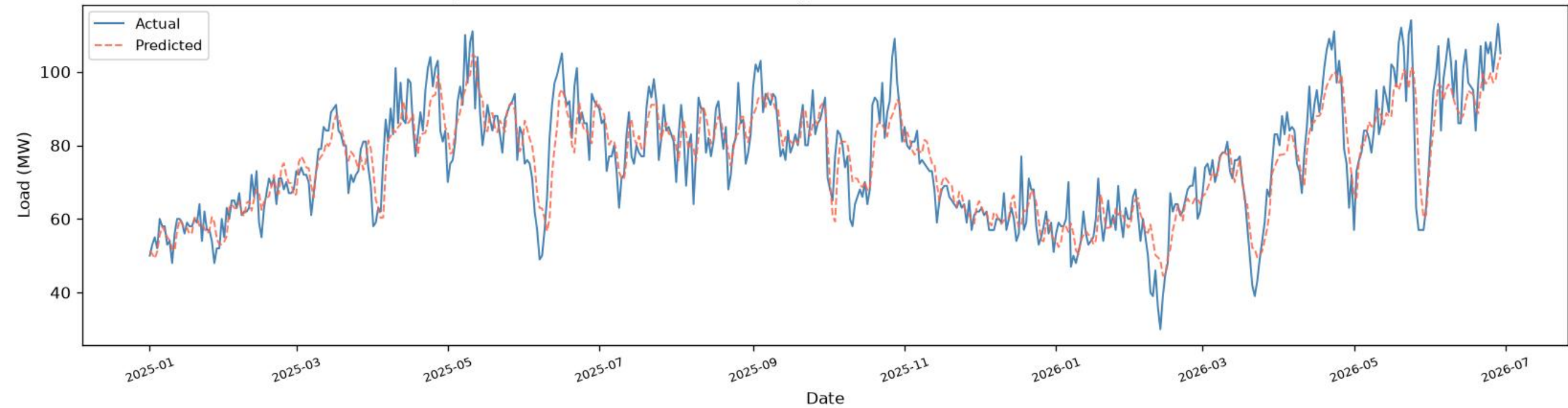
Uttara | BiGRU+BiLSTM - TEST ( \geq 2025 ), one-day-ahead ( R^2=0.8165 , RMSE=6.91 , MAE=5.24 , n=536 )
