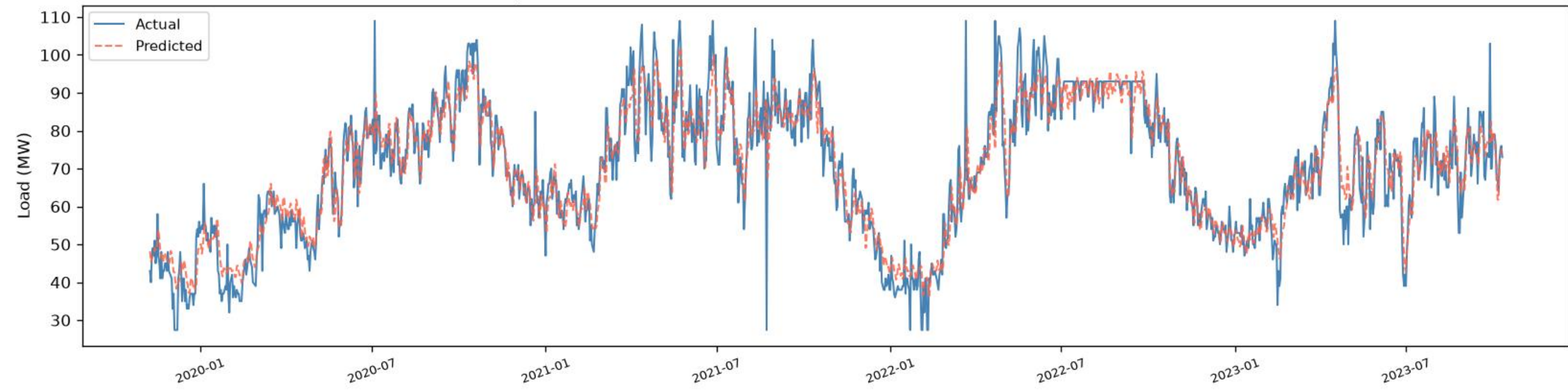
Uttara | BiGRU+BiLSTM - TRAIN (fit block) ( R^2=0.8781 , RMSE=6.15, MAE=4.38, n=1383 )
