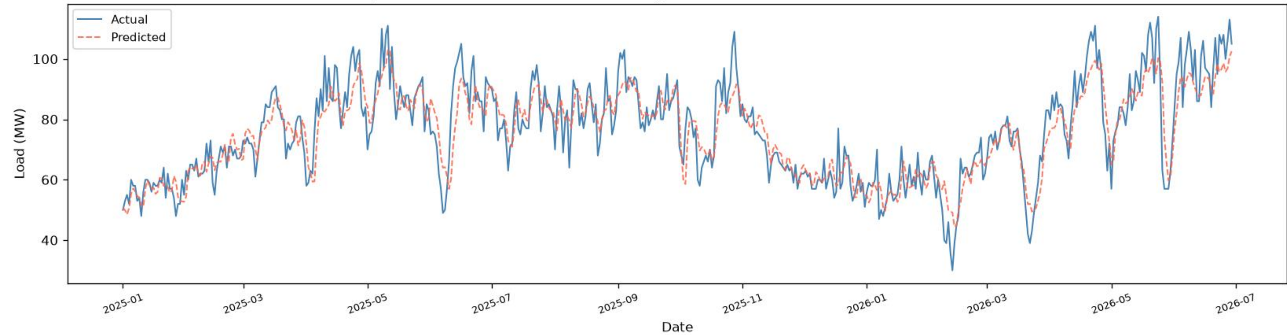
Uttara | BiLSTM+BiGRU - TEST ( \geq 2025 ), one-day-ahead ( R^2=0.8053 , RMSE=7.11 , MAE=5.40 , n=536 )
