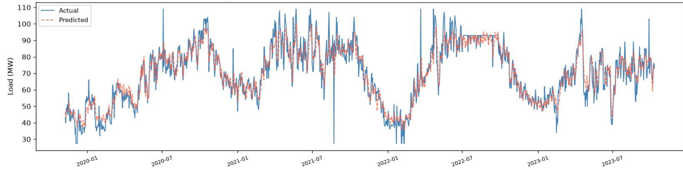
Uttara | BiLSTM+BiGRU - TRAIN (fit block) ( R^2=0.8763 , RMSE=6.20, MAE=4.43, n=1383 )
