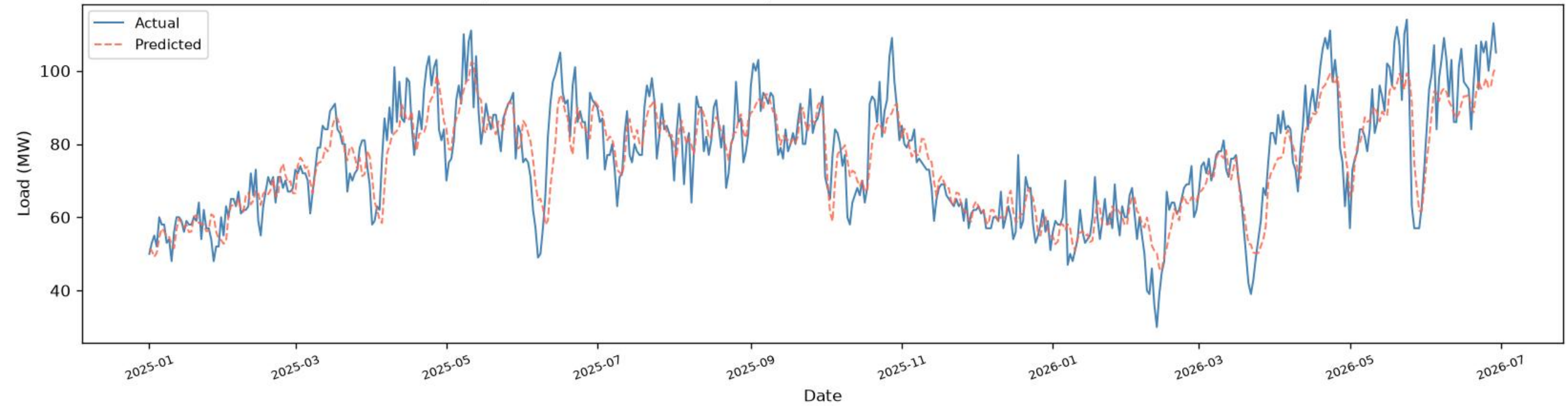
Uttara | BiLSTM - TEST ( \geq 2025 ), one-day-ahead ( R^2=0.7911 , RMSE=7.37 , MAE=5.57 , n=536 )
