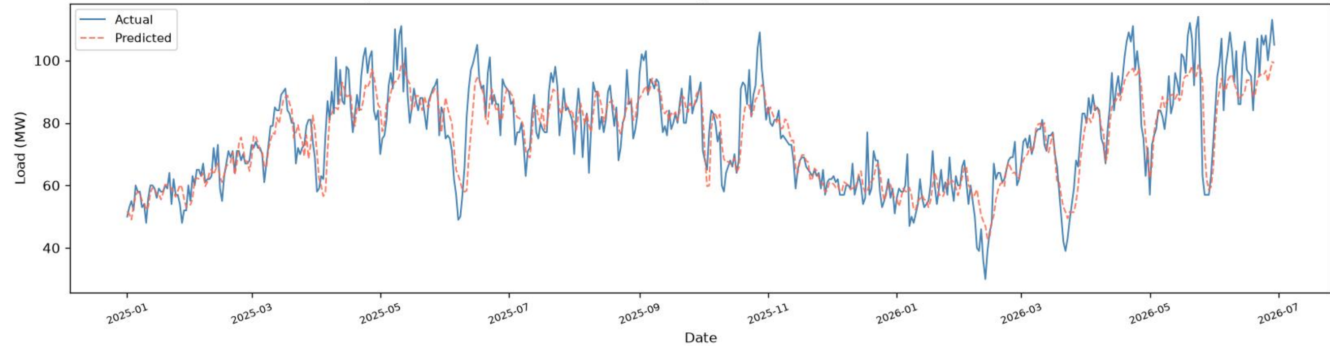
Uttara | CNN+BiGRU+BiLSTM - TEST ( \geq 2025 ), one-day-ahead ( R^2=0.8172 , RMSE=6.89 , MAE=5.14 , n=536 )
