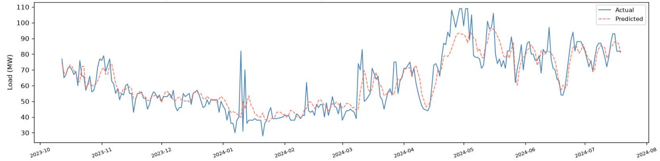
Uttara | CNN+BiGRU+BiLSTM - VALIDATION (chronological, before test) ( R^2=0.8143 , RMSE=7.94, MAE=5.66, n=272 )
