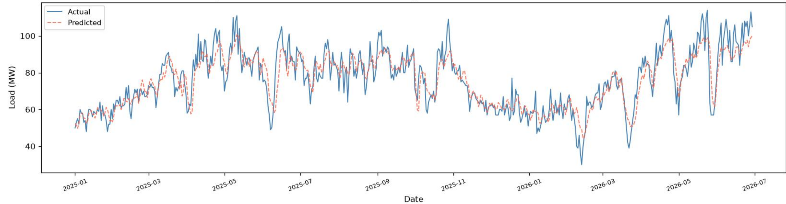
Uttara | CNN+BiLSTM+BiGRU - TEST ( \geq 2025 ), one-day-ahead ( R^2=0.7977 , RMSE=7.25 , MAE=5.45 , n=536 )
