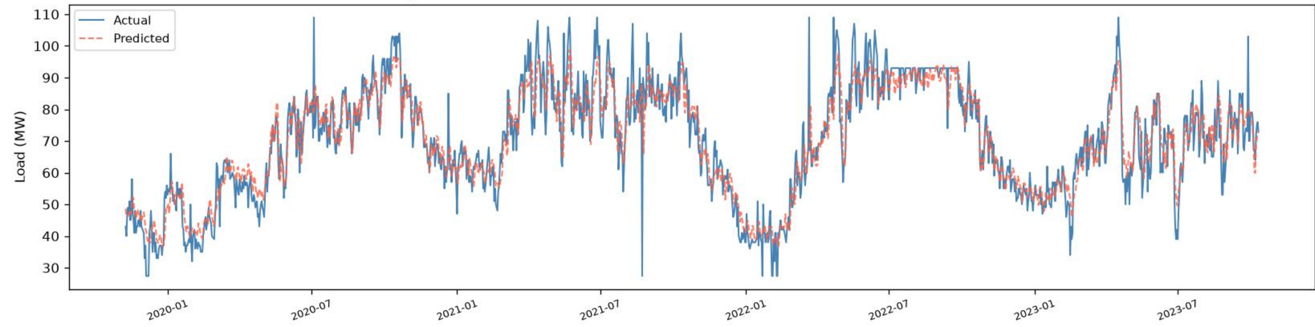
Uttara | CNN+BiLSTM+BiGRU - TRAIN (fit block) (R2=0.8768, RMSE=6.19, MAE=4.46, n=1383)
