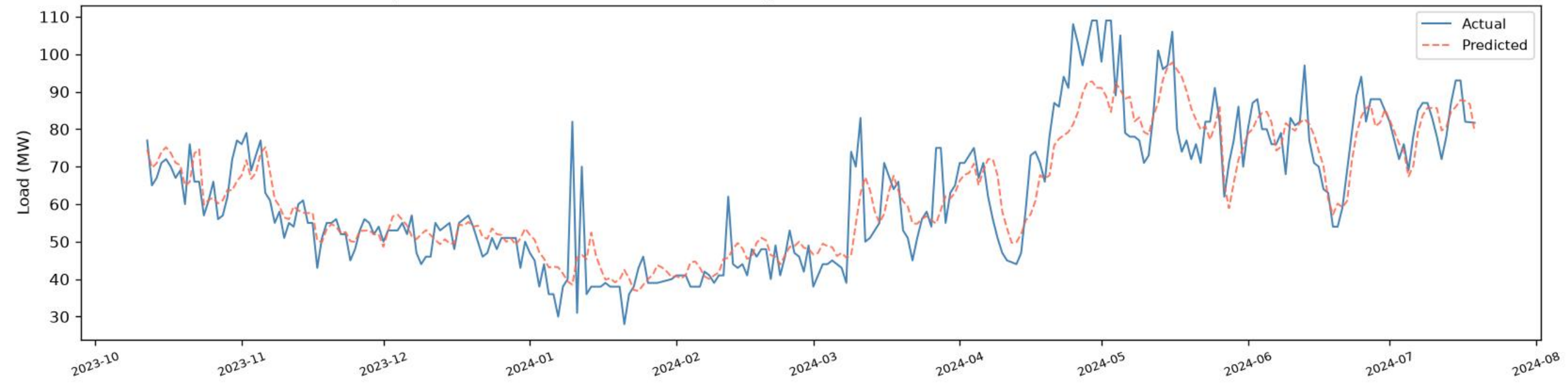
Uttara | CNN+BiLSTM+BiGRU - VALIDATION (chronological, before test) ( R^2=0.7986 , RMSE=8.26, MAE=6.02, n=272 )
