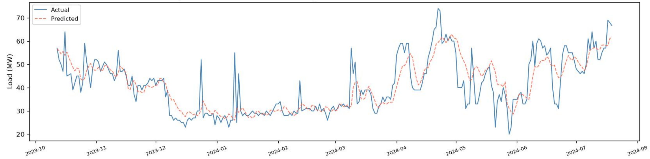
Uttara New | BiGRU+BiLSTM - VALIDATION (chronological, before test) ( R^2=0.6630 , RMSE=6.80 , MAE=4.70 , n=269 )
