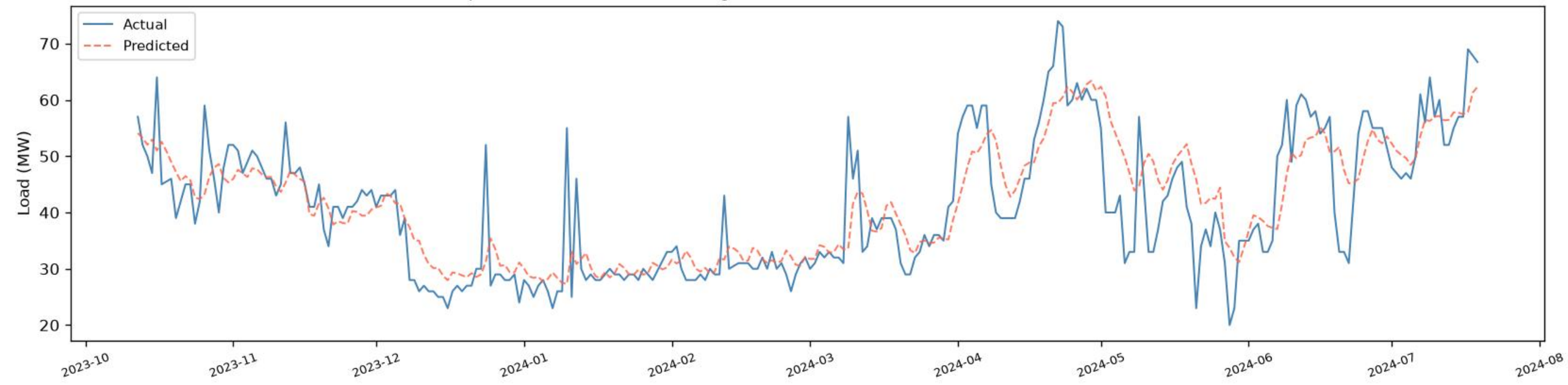
Uttara New | BiGRU - VALIDATION (chronological, before test) (R2=0.6663, RMSE=6.77, MAE=4.75, n=269)
