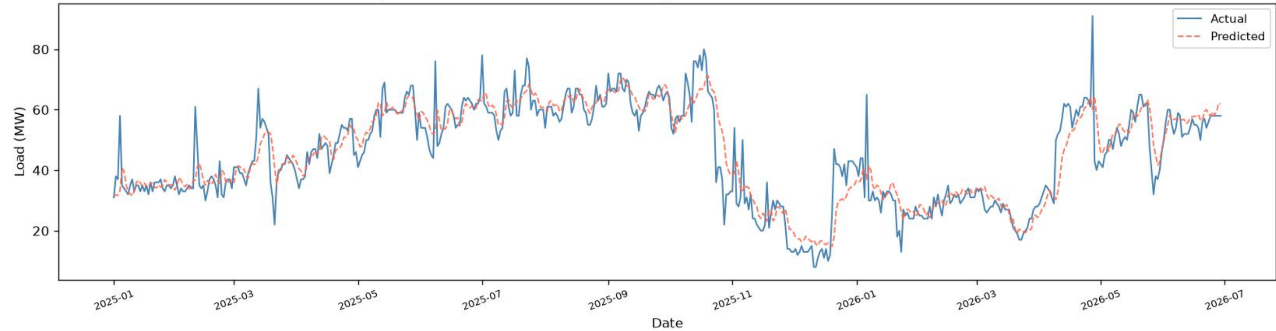
Uttara New | BiLSTM+BiGRU - TEST ( \geq 2025 ), one-day-ahead ( R^2=0.8381 , RMSE=6.50 , MAE=4.44 , n=531 )
