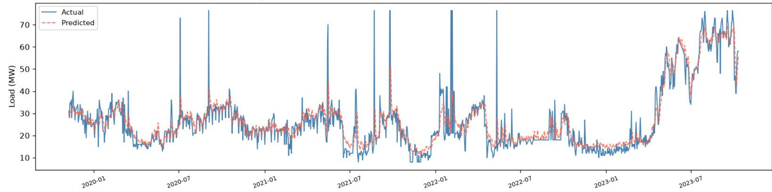
Uttara New | BiLSTM+BiGRU - TRAIN (fit block) (R2=0.8136, RMSE=6.09, MAE=3.52, n=1346)
