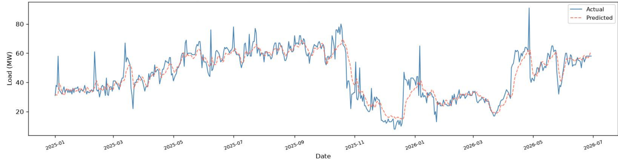
Uttara New | BiLSTM - TEST ( \geq 2025 ), one-day-ahead ( R^2=0.8308 , RMSE=6.64 , MAE=4.49 , n=531 )
