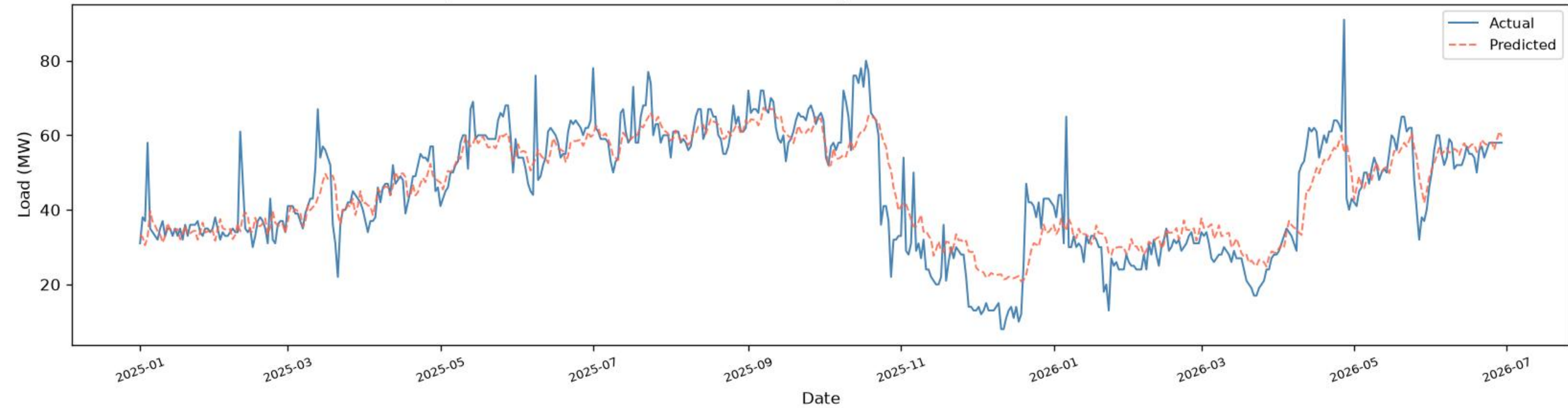
Uttara New | CNN+BiGRU+BiLSTM - TEST ( \geq 2025 ), one-day-ahead ( R^2=0.8007 , RMSE=7.21 , MAE=5.15 , n=531 )
