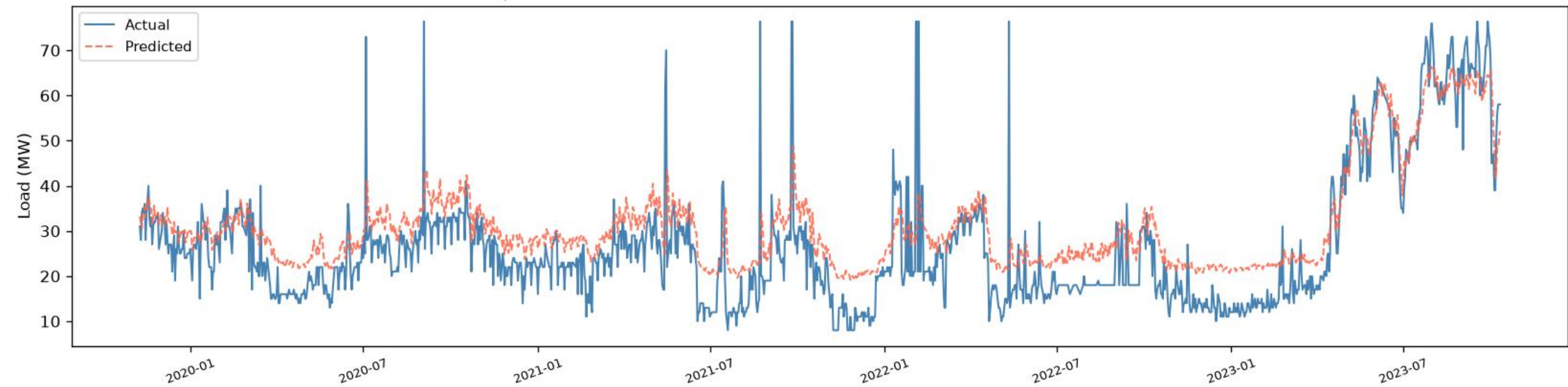
Uttara New | CNN+BiGRU+BiLSTM - TRAIN (fit block) (R2=0.6832, RMSE=7.94, MAE=6.42, n=1346)
