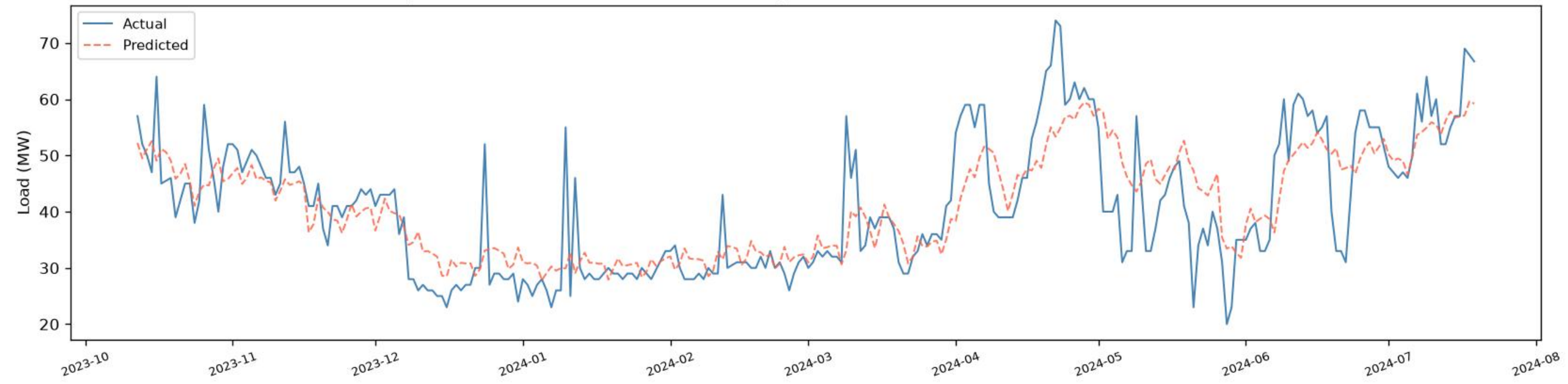
Uttara New | CNN+BiGRU+BiLSTM - VALIDATION (chronological, before test) ( R^2=0.6308 , RMSE=7.12, MAE=5.21, n=269 )
