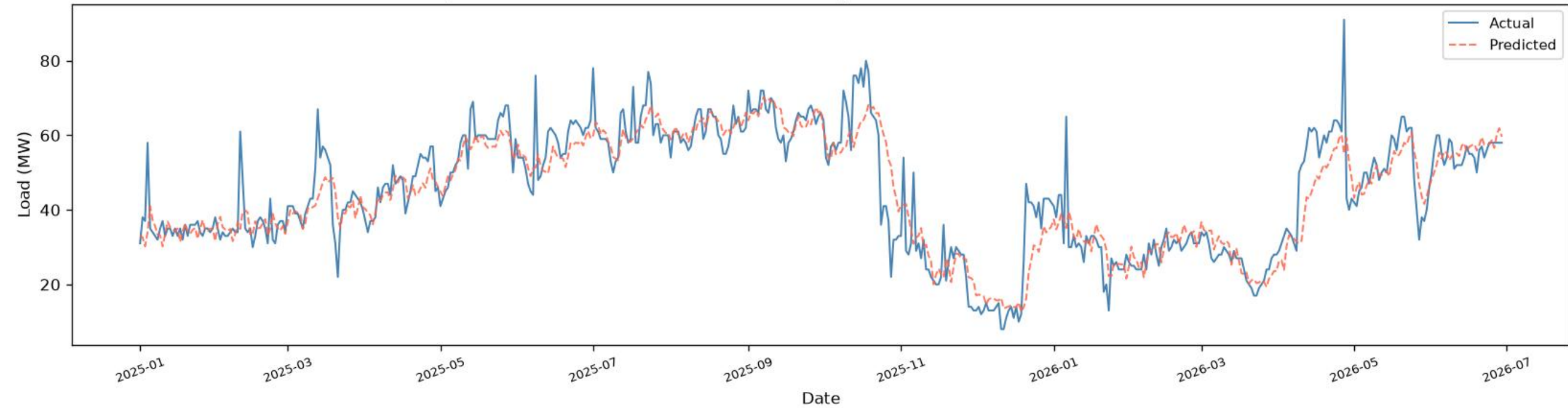
Uttara New | CNN+BiLSTM+BiGRU - TEST ( \geq 2025 ), one-day-ahead ( R^2=0.8207 , RMSE=6.84 , MAE=4.63 , n=531 )
