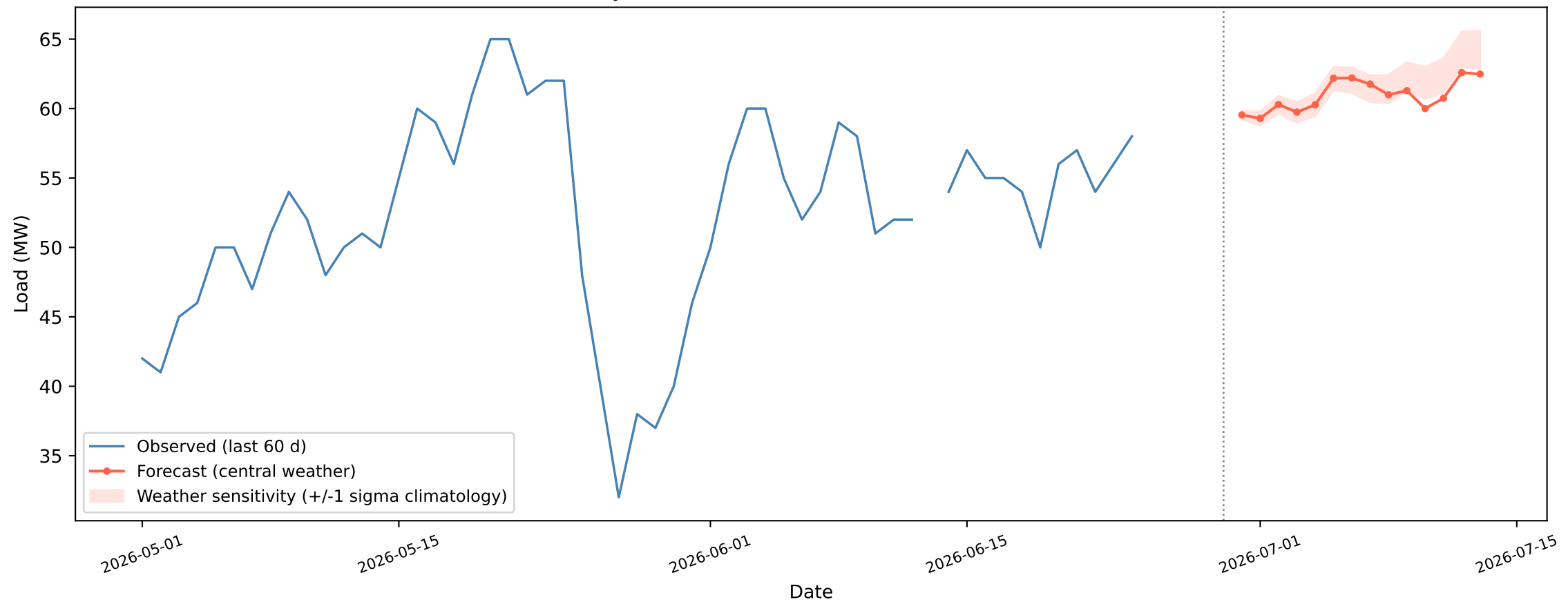
Uttara New - 14-day recursive forecast (BiGRU), weather mode = forecast
