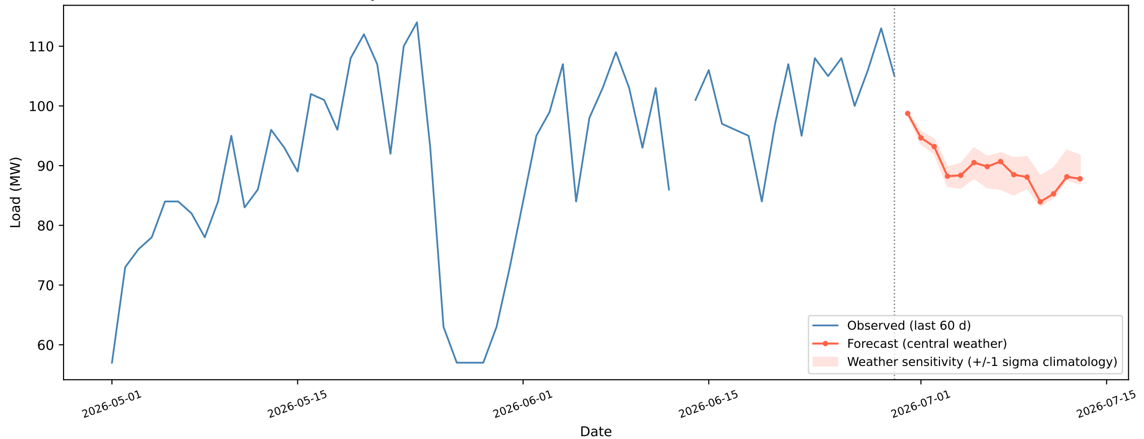
Uttara - 14-day recursive forecast (CNN+BiGRU+BiLSTM), weather mode = forecast
