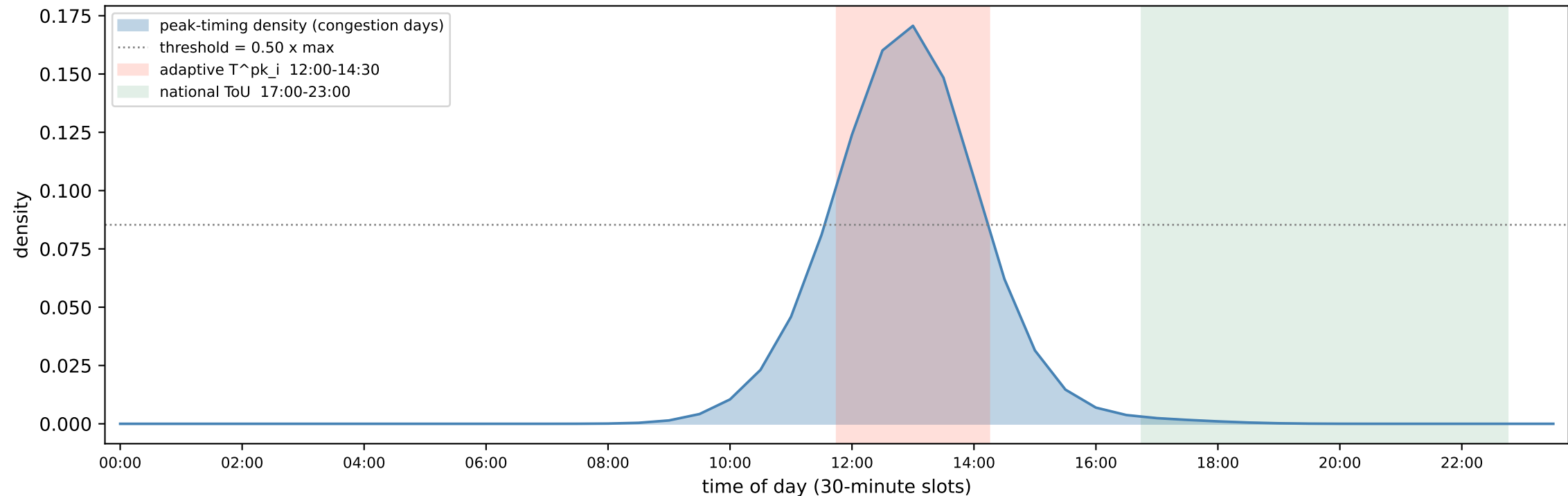
Dhanmondi - when this substation peaks on its 121 most congested days
