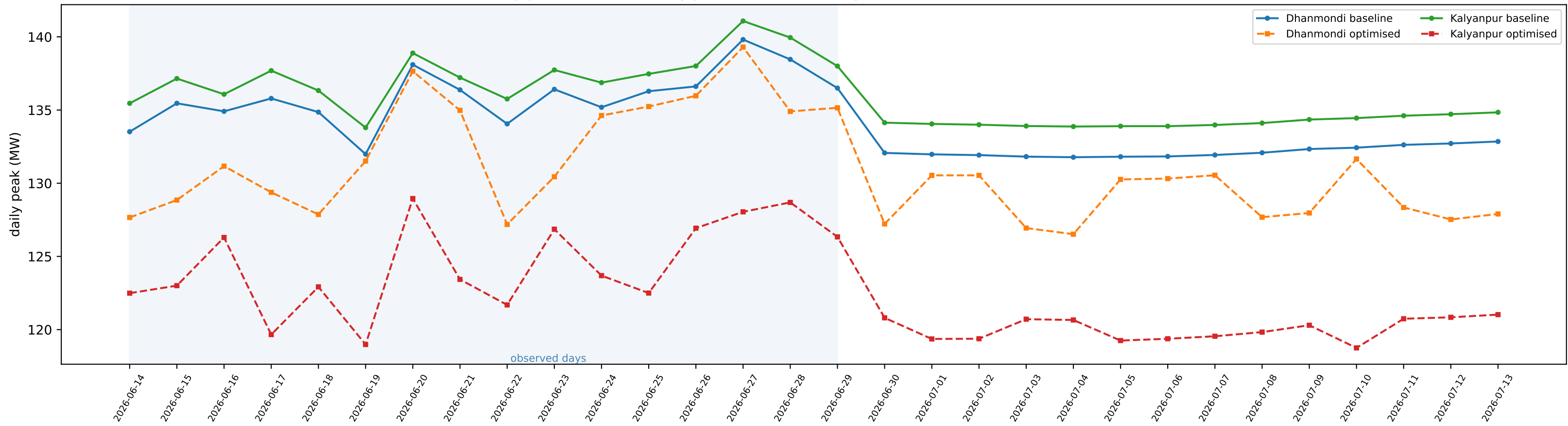
Daily peak over the billing period, baseline vs optimised (2026-06-14 to 2026-07-13)
