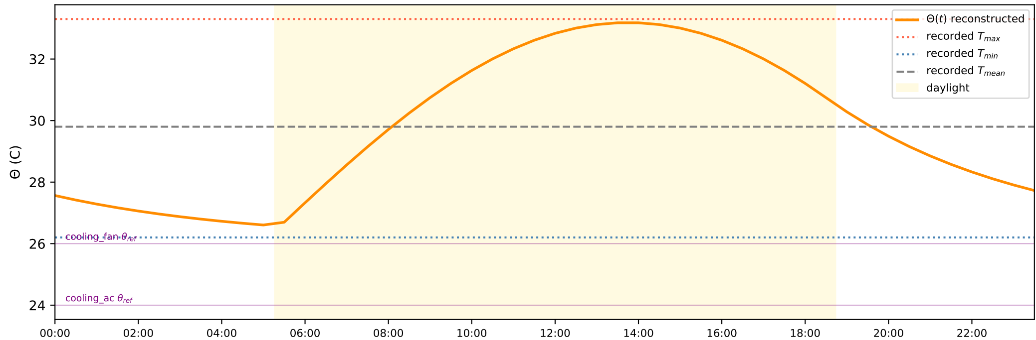
Reconstructed diurnal temperature, 2026-06-29 (Parton-Logan, mean-corrected)
