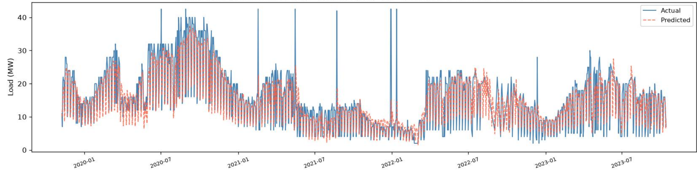
Bangabhaban | CNN+BiLSTM+BiGRU - VALIDATION (chronological, before test) (R2=0.5665, RMSE=3.93, MAE=2.80, n=210)
