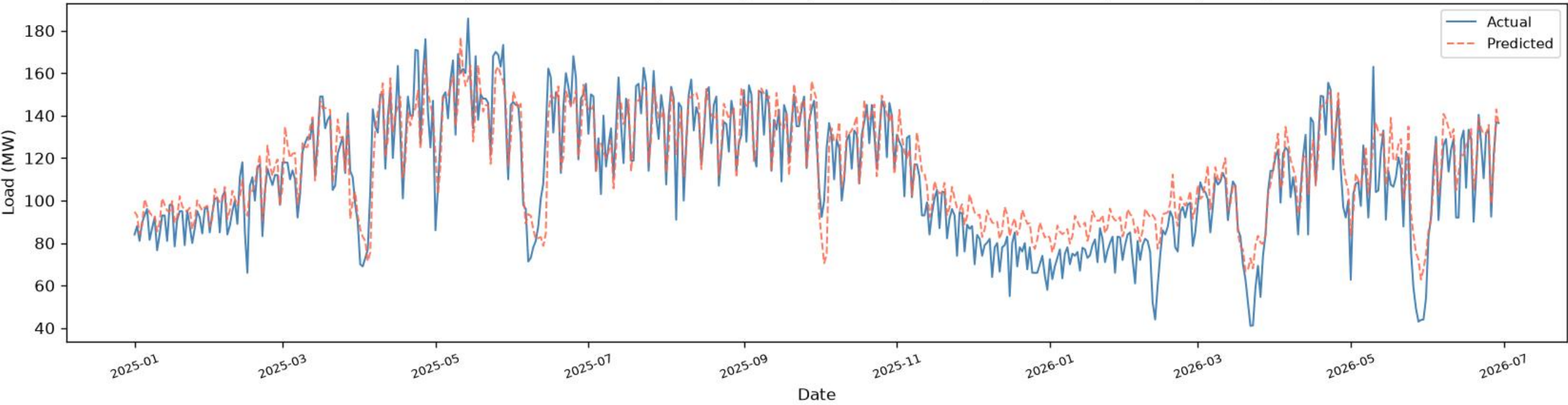
Dhanmondi | BiLSTM+BiGRU - TEST (>= 2025), one-day-ahead (R2=0.8174, RMSE=12.57, MAE=9.72, n=536)
