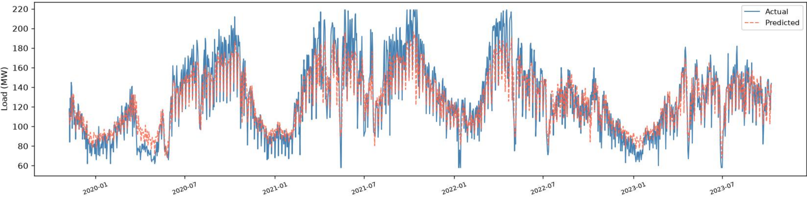
Dhanmondi | BiLSTM+BiGRU - VALIDATION (chronological, before test) (R2=0.7134, RMSE=15.94, MAE=10.95, n=271)
