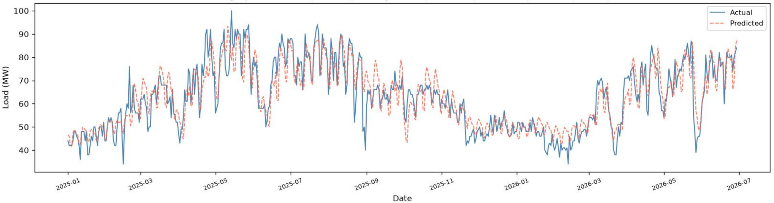
Maniknagar | BiLSTM - TEST (>= 2025), one-day-ahead (R2=0.7895, RMSE=6.63, MAE=5.05, n=525)
