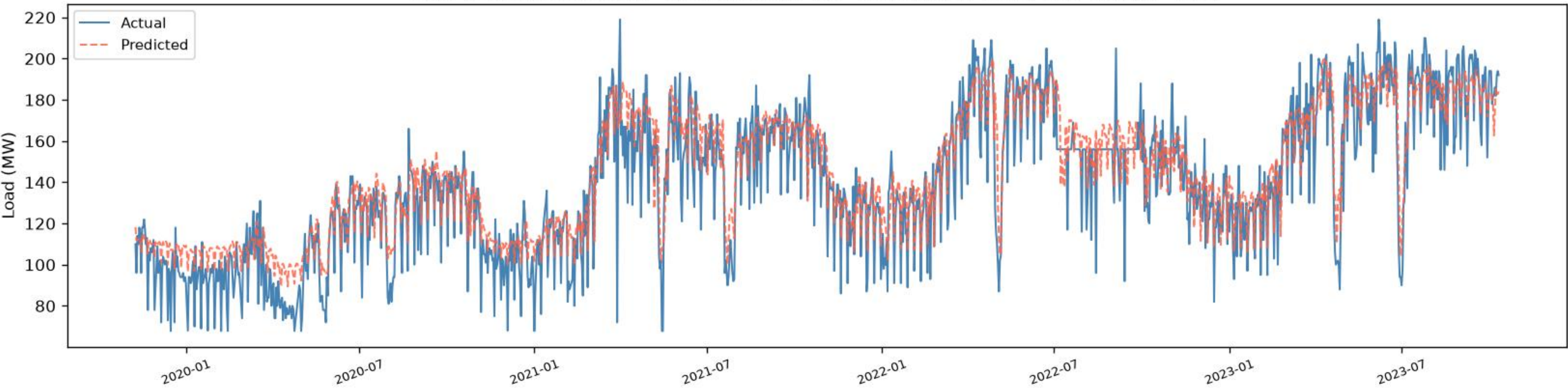
Savar | CNN+BiGRU+BiLSTM - VALIDATION (chronological, before test) (R2=0.7086, RMSE=18.68, MAE=13.31, n=272)
