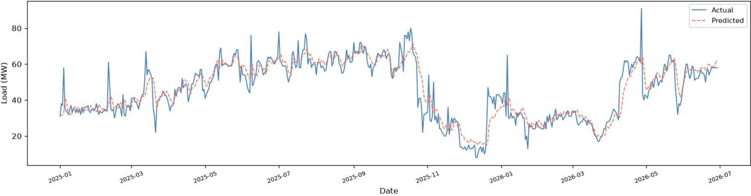
Uttara New | BiLSTM+BiGRU - TEST (>= 2025), one-day-ahead (R2=0.8381, RMSE=6.50, MAE=4.44, n=531)
