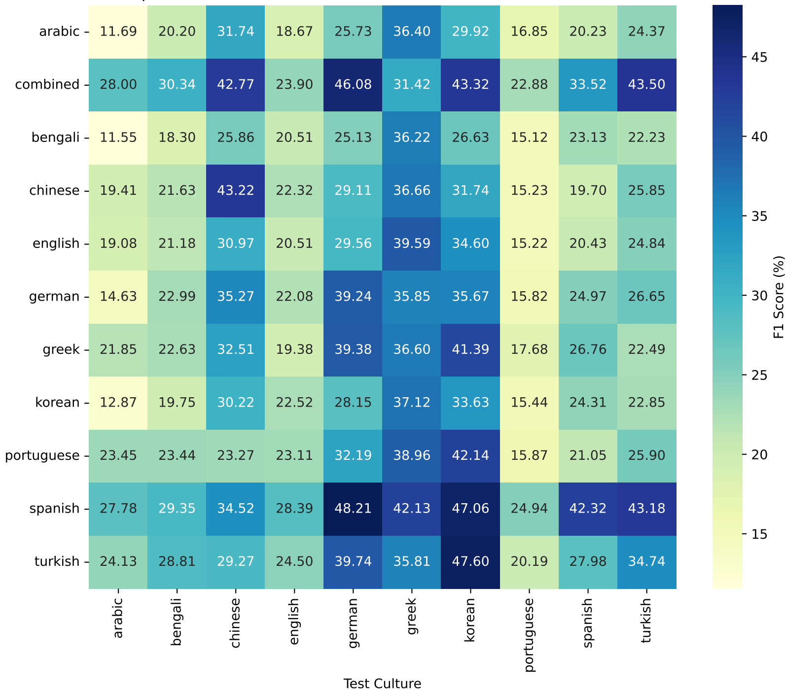
Adapter Performance Across Cultures for Meta-Llama-3.1-8B-Instruct
