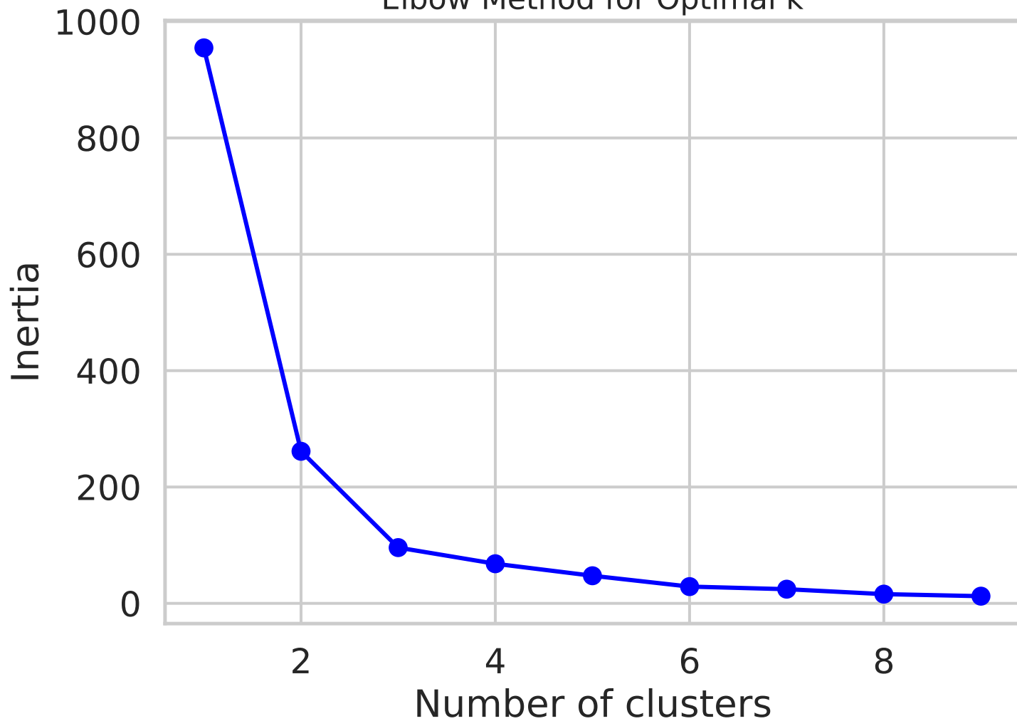
Elbow Method for Optimal k
