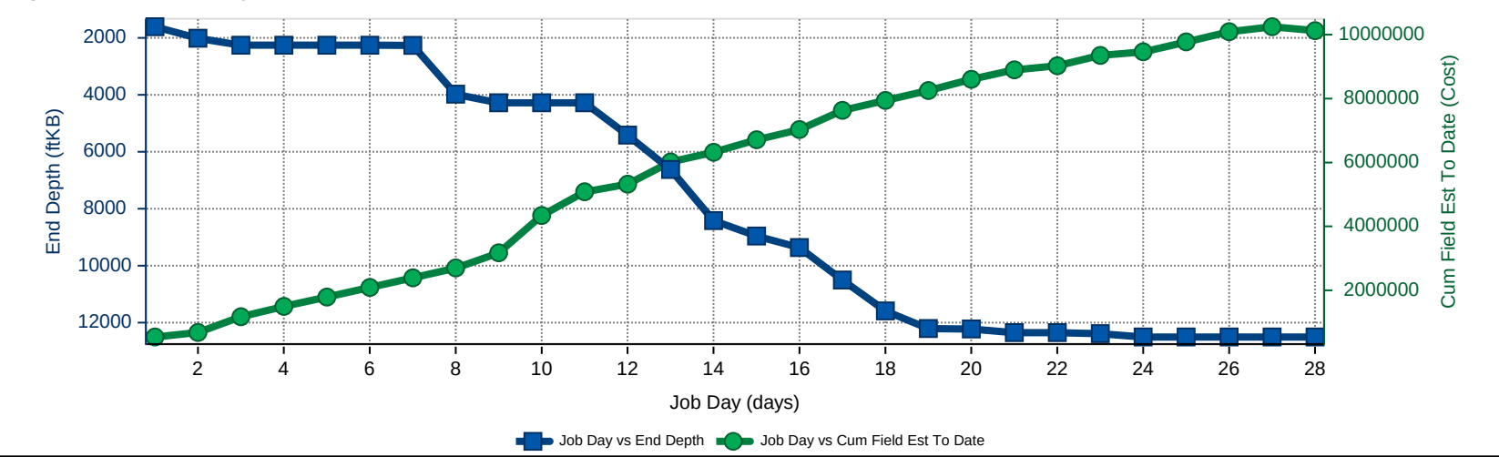
Depth and Cost vs Days
