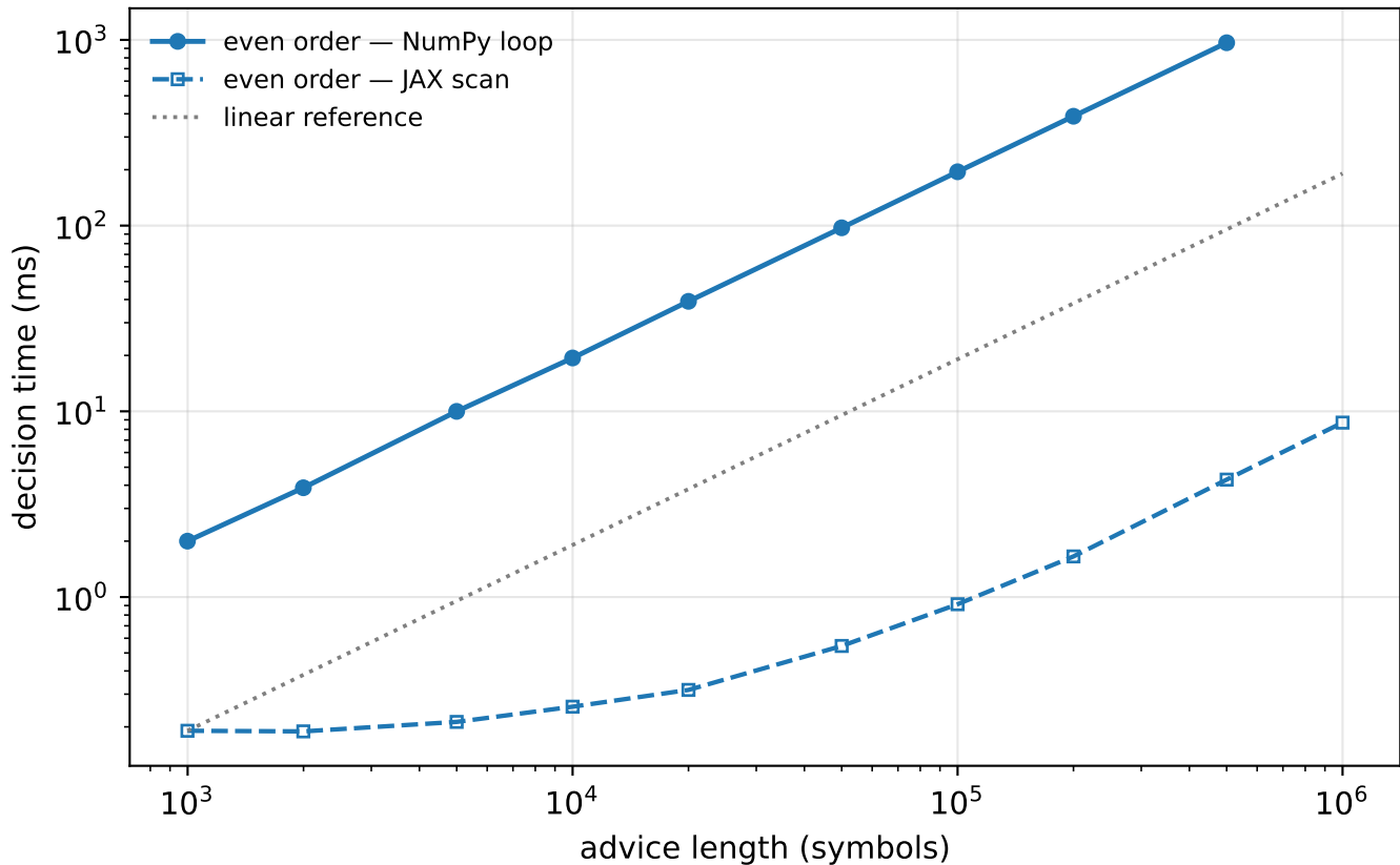
Deciding even order across all finite abelian groups
