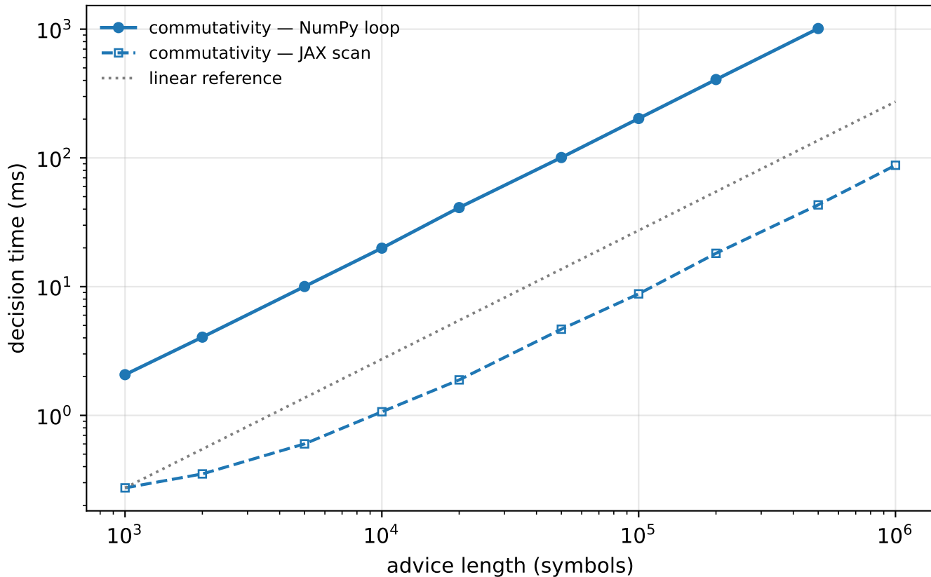
Deciding commutativity in extraspecial 3-groups
