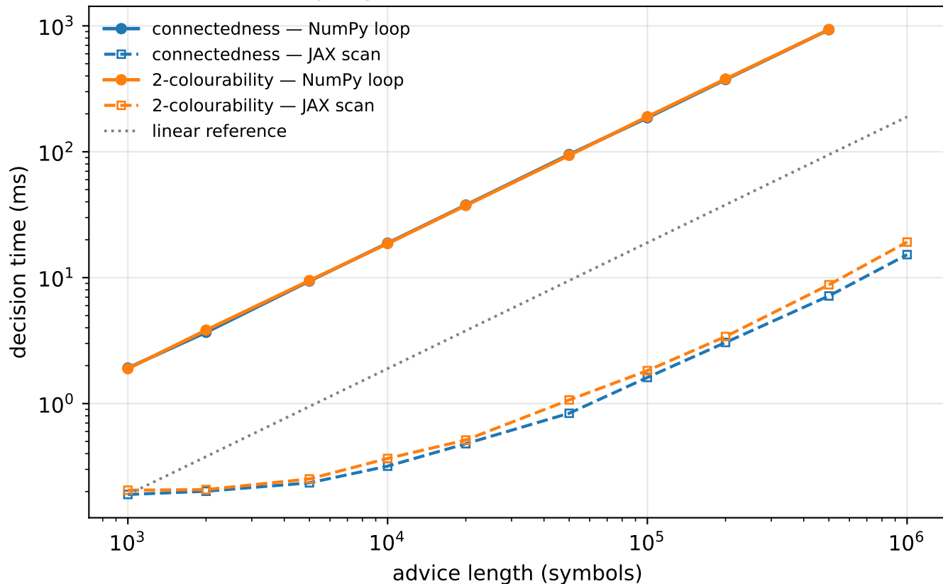
MSO query evaluation on PathWidthClass(2)
