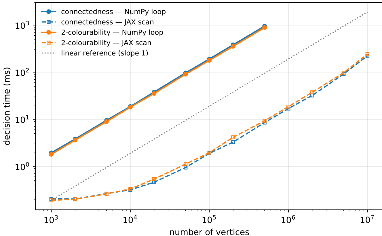
Linear-time MSO query evaluation on TreeDepthClass(4)
