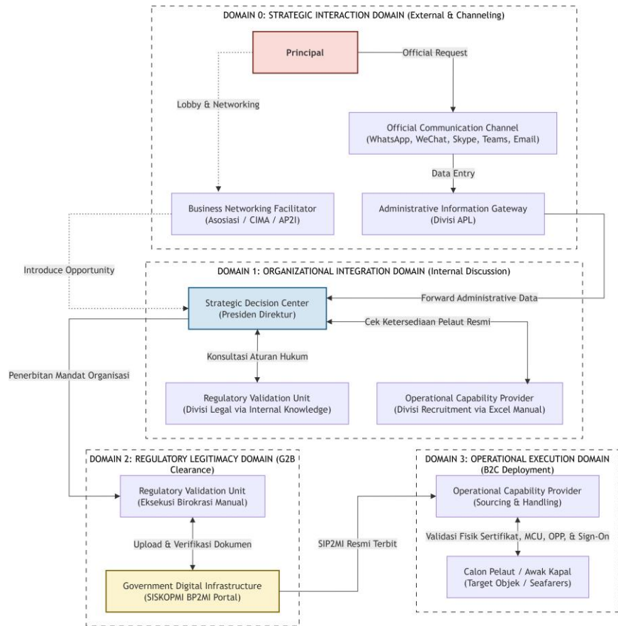
Gambar 5 Artifak Peta Diagram awal Non-Disiplin-UML
