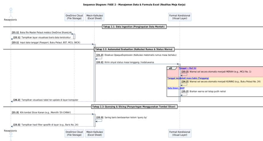
Gambar 22 Diagram Sequences Phase 2
