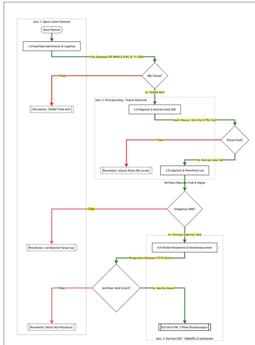
Gambar 13 Flowchart Mikro
