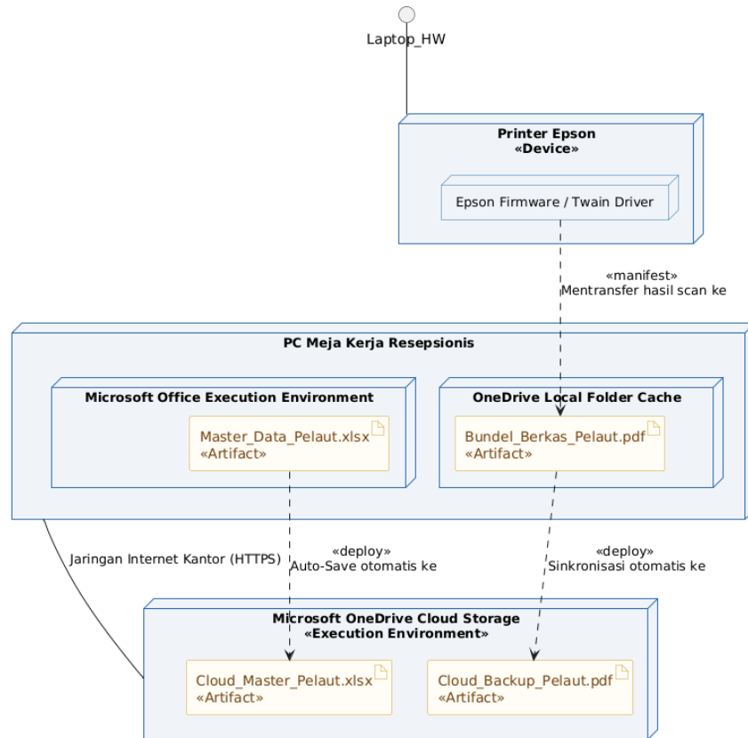
Deployment Diagram Jayus: Topologi Fisik & Artefak Alat Tempur Kantor
