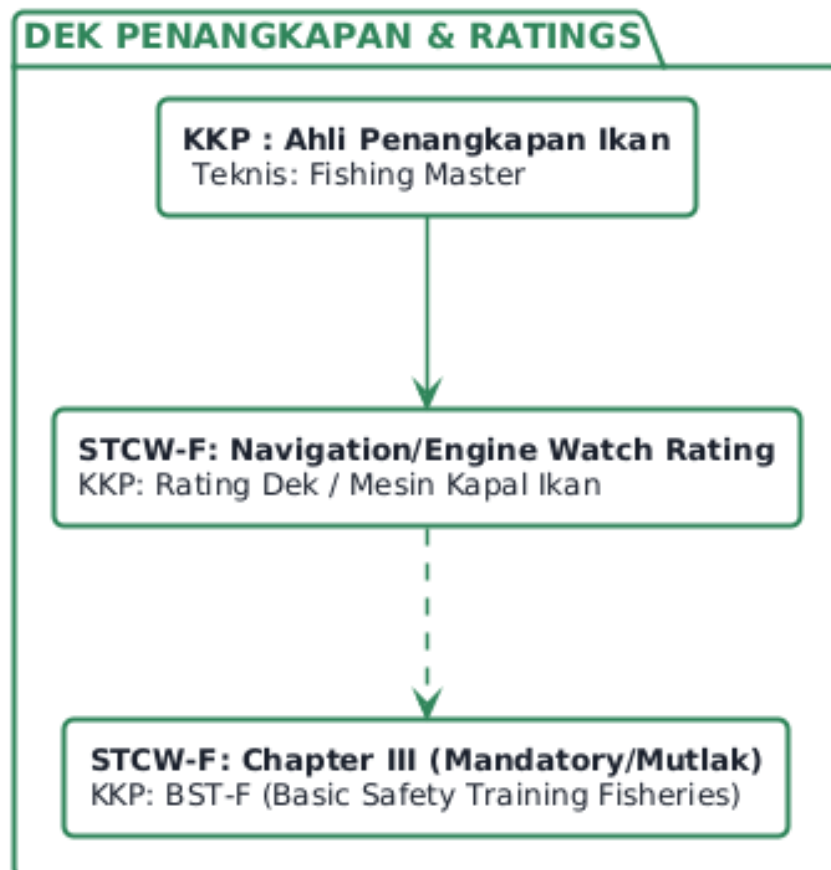
Gambar 11 STCW-F & KKP Nomenklatur Nautika Dek & Dokumen Mutlak F Series
