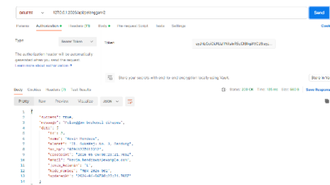
Gambar 2.12 DELETE Pelanggan
