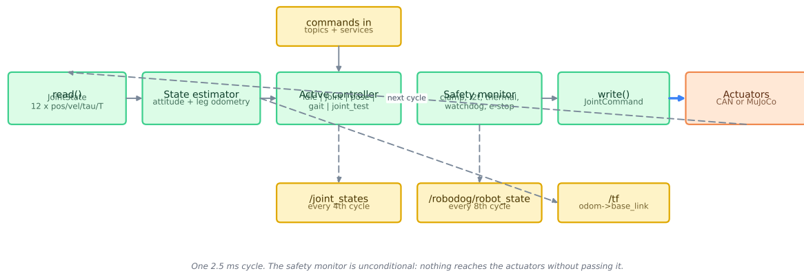
Figure 6: One 400 Hz cycle. The safety monitor is unconditional.
