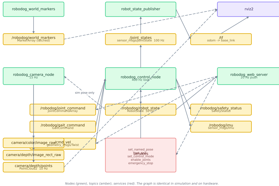
Figure 4: Node and topic graph. Identical in simulation and on hardware; only the implementations behind the two backends differ.
