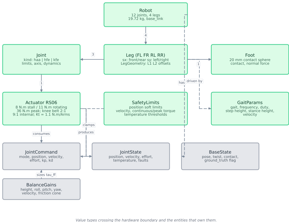
Figure 12: Domain model: the value types that cross the hardware boundary and the entities that own them.
