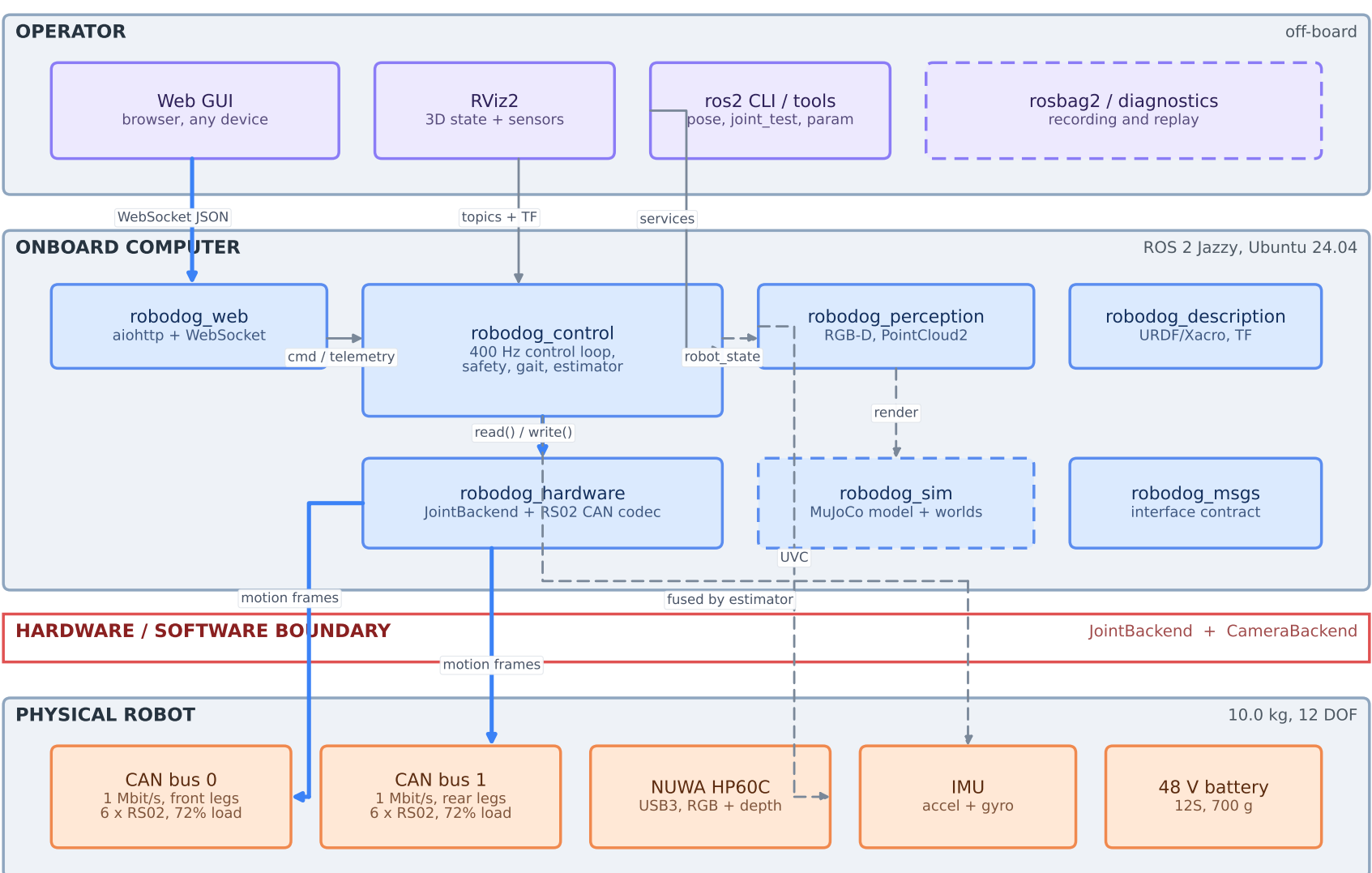
Physical and computational stack. Everything above the red boundary is identical in simulation and on hardware.
