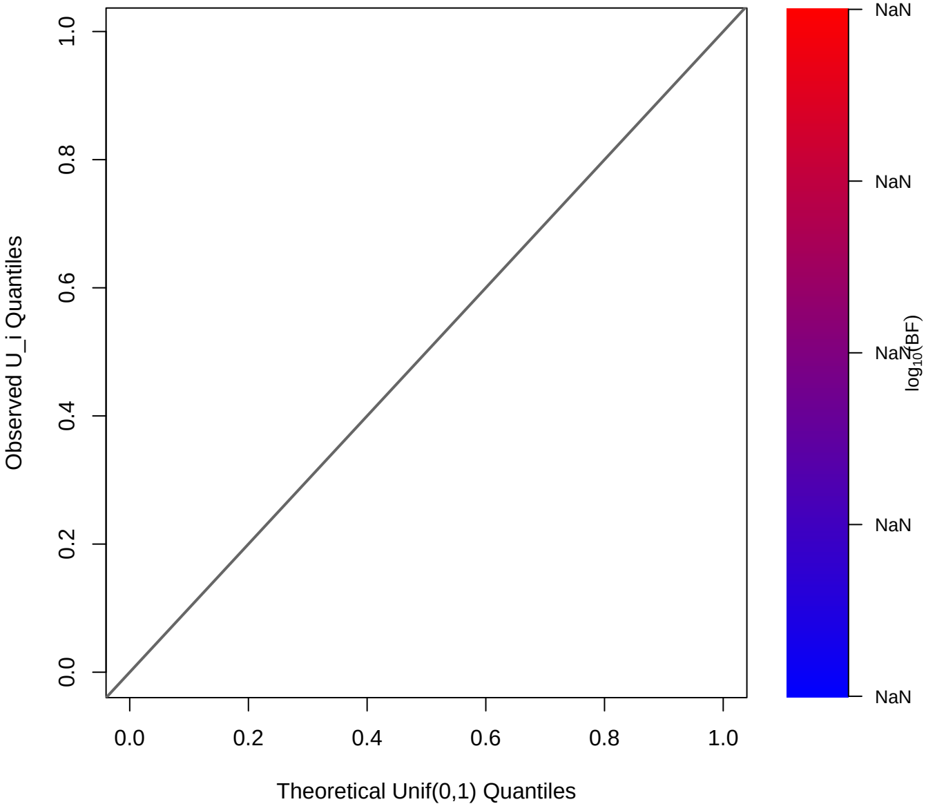
Diagnostic QQ-Plot
