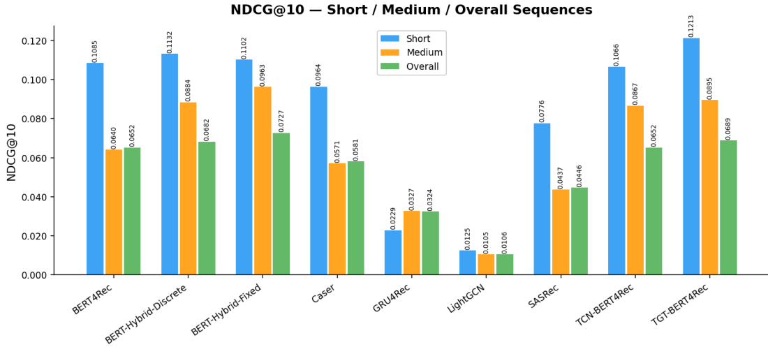
Figure 3.4: NDCG@10 by user history length group on ML-1M.
