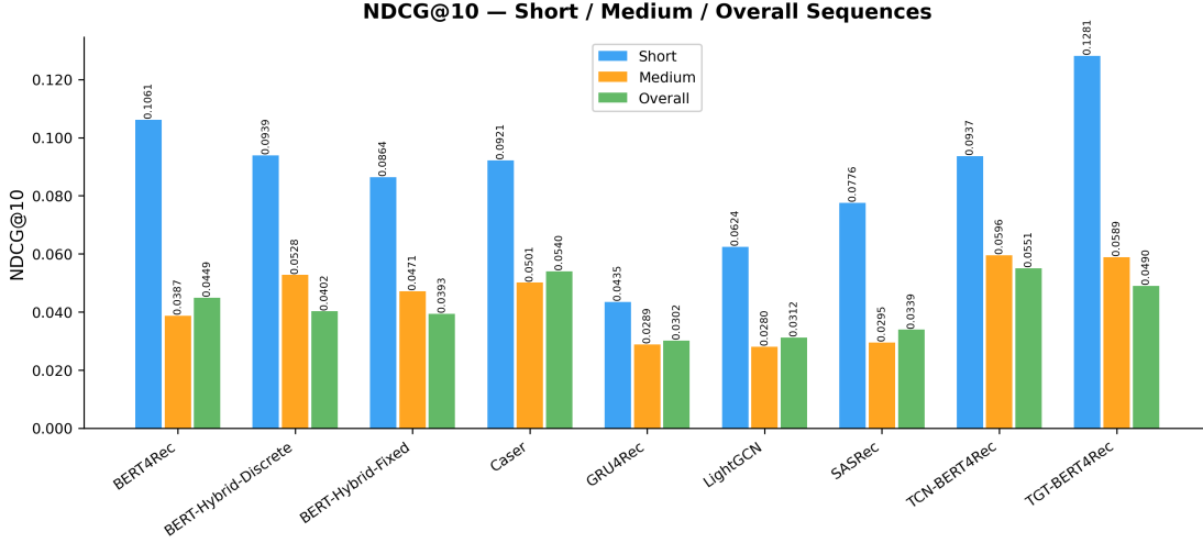
Figure 3.5: NDCG@10 by user history length group on ML-100K.
