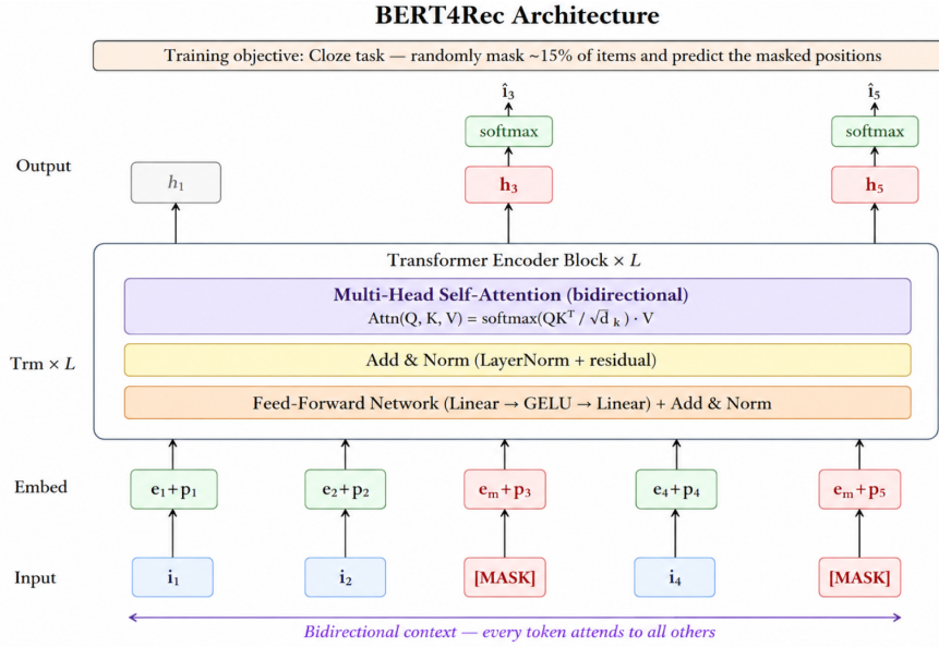
Figure 1.3: Architecture of a Transformer-based sequential model (SASRec/BERT4Rec).
