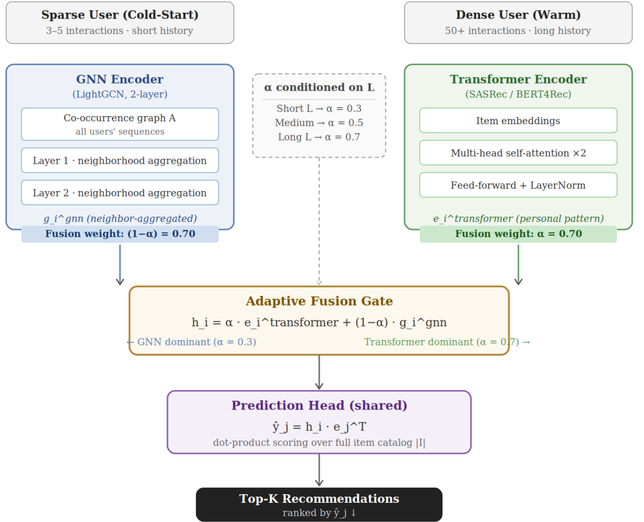
Figure 2.1: Proposed Architecture of the Length-Adaptive Hybrid GNN-Transformer.
